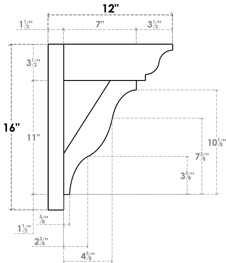
SIDE PROFILE
